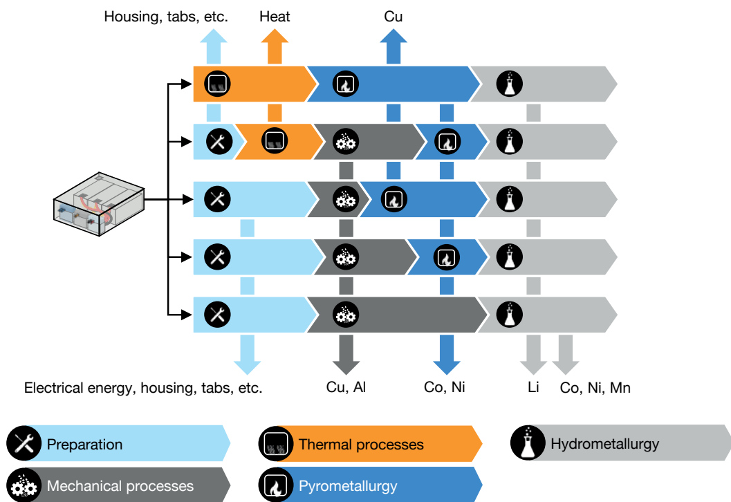
Figure 28: Recovered materials in the different recycling stages; Source: PEM of RWTH Aachen University
