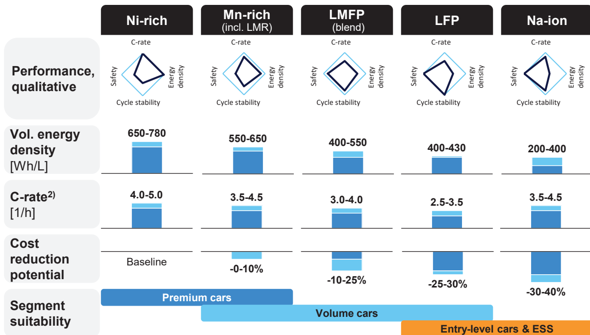
Figure 8: Comparison of cell technologies by cathode chemistry on cell level 1) – cost reduction potential depending on raw material prices; Source: Announcements from cell manufacturers, interviews with market participants, press clippings, Roland Berger
