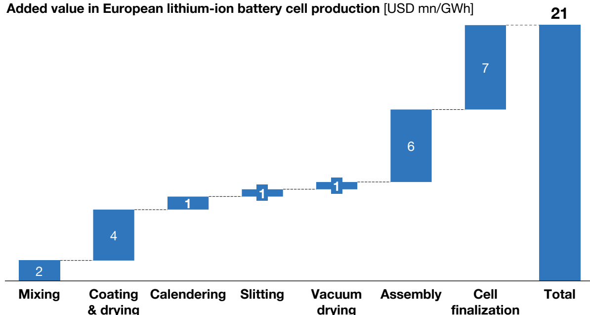
Figure 12: Added value structure in lithium-ion battery production in Europe; Source: PEM of RWTH Aachen University Production Model
