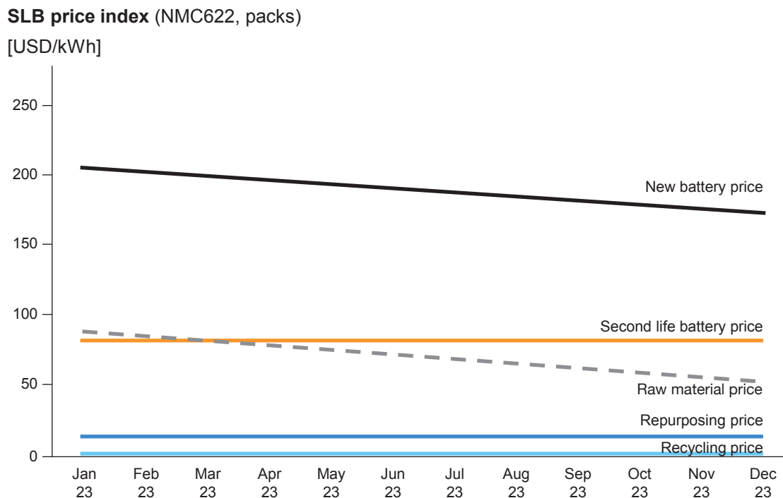
Figure 29: Battery pack-level prices from the current price index for SLBs (NMC622 cathode chemistry); Source: PEM of RWTH Aachen University
