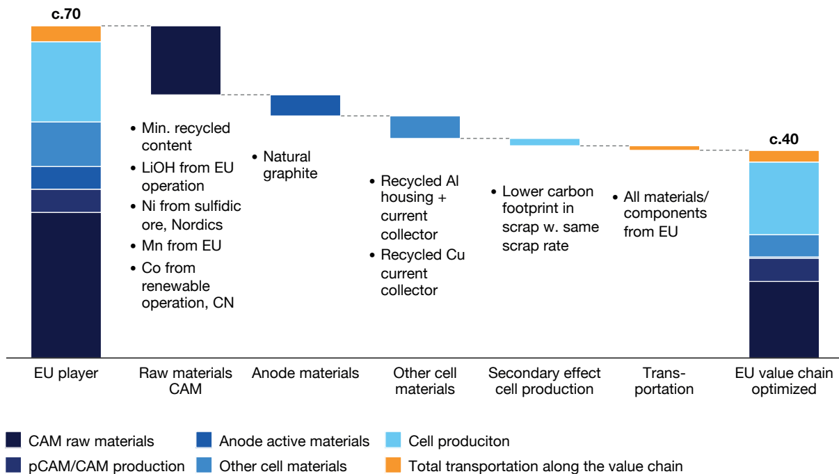
Figure 7: Carbon footprint optimization for value chain levers; Source: Roland Berger LiB cell carbon footprint model
